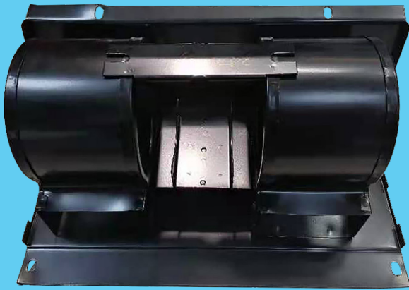
DC001 KW Blower Motor Assembly
